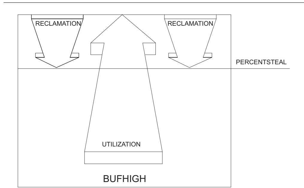
Figure 31. Bufhigh utilization with percentsteal
