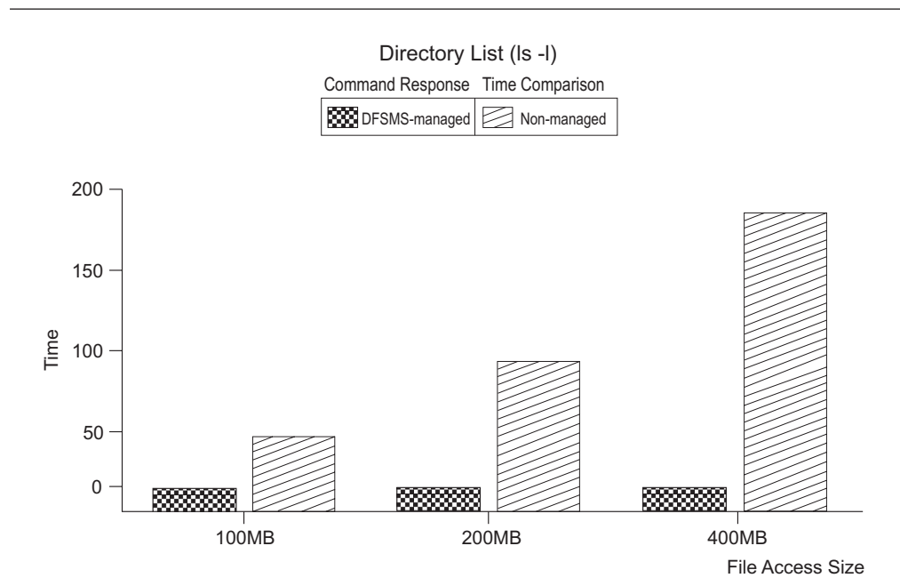
Figure 30. Directory list comparison between DFSMS-managed and non-managed
