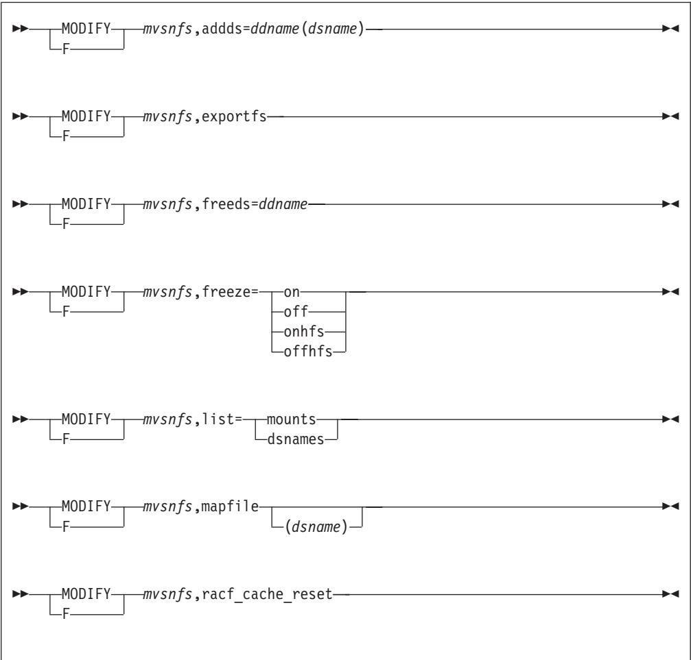
Figure 24. Summary of the modify command (Part 1 of 2)
